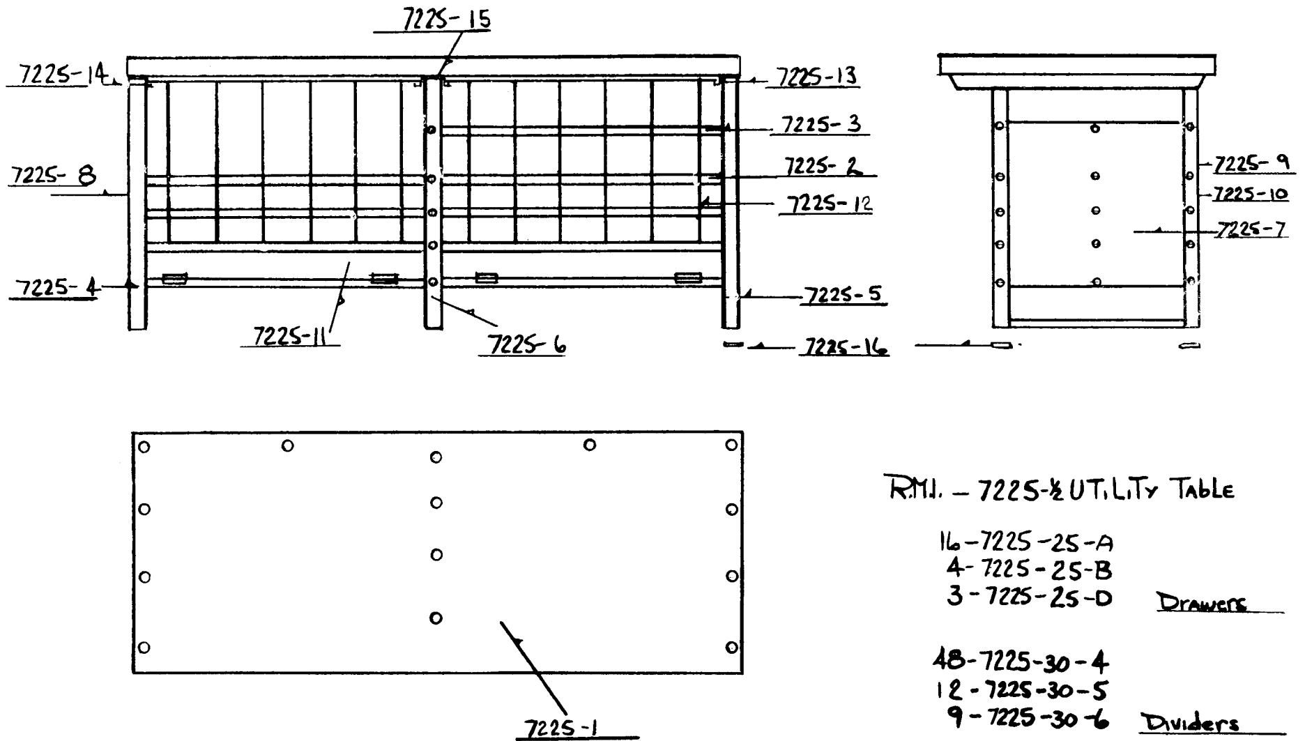
Figure 1. Breakdown of work table, model 7225.
